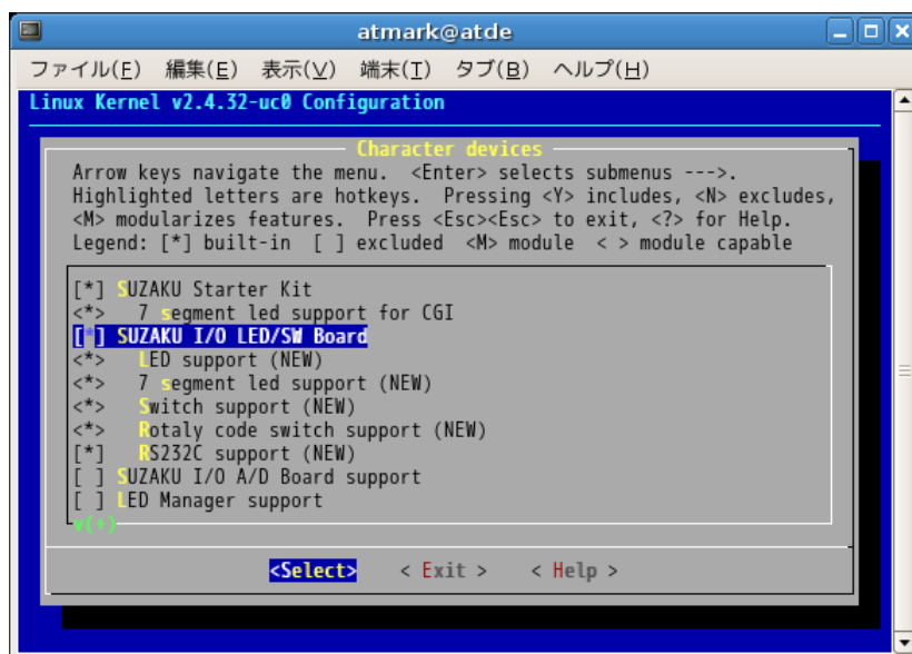
図 8-2 Character devices
