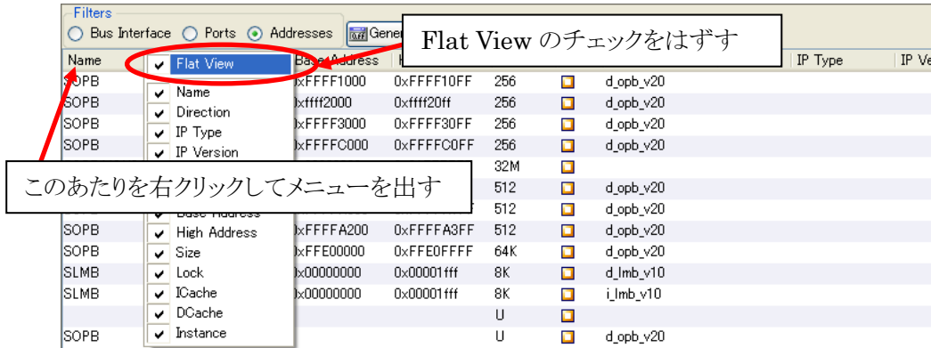
図 10-74 Flat View
