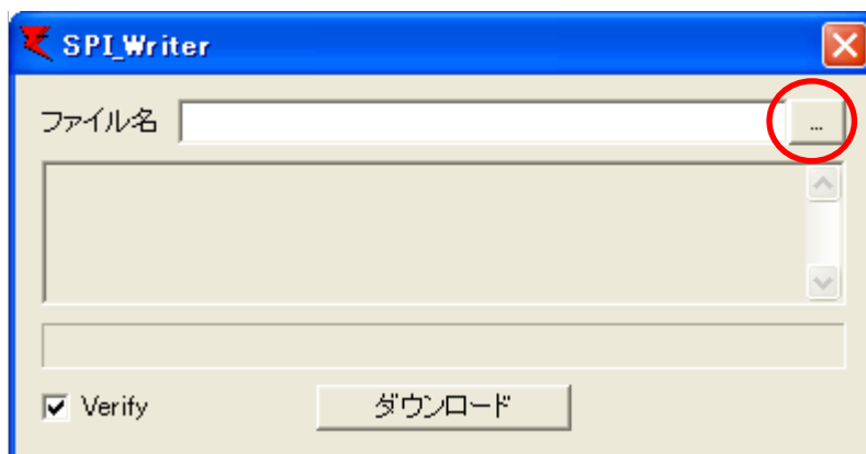
図 6-28 SPI_Writer
