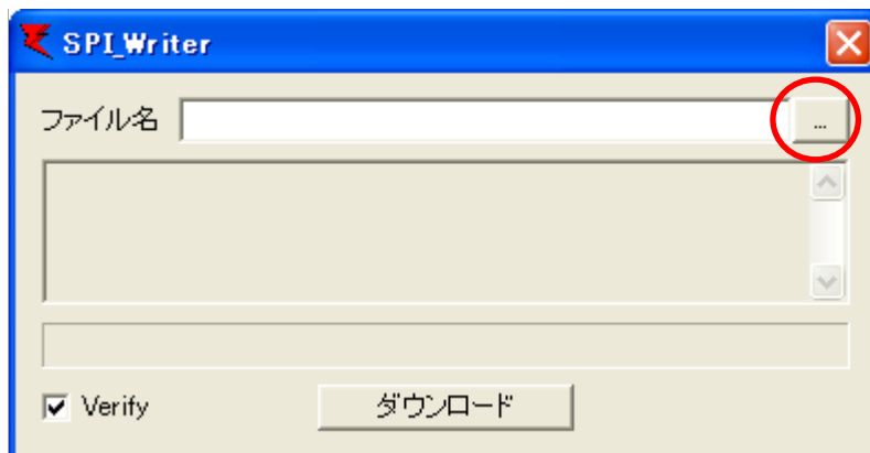
図 6-26 SPI_Writer
