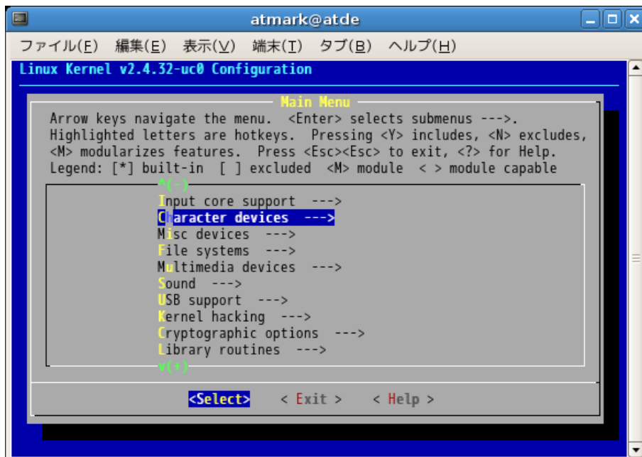
図 8.2 Character devices
