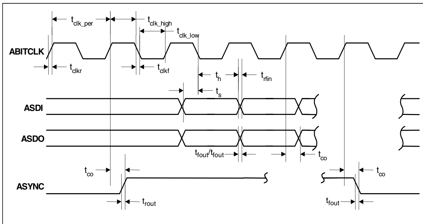
Figure 36. AC '97 Configuration Timing Measurement
