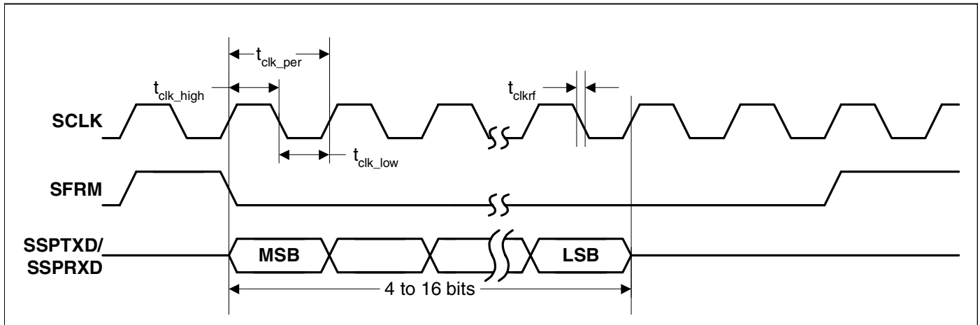
Figure 32. SPI Single Transfer Timing Measurement
