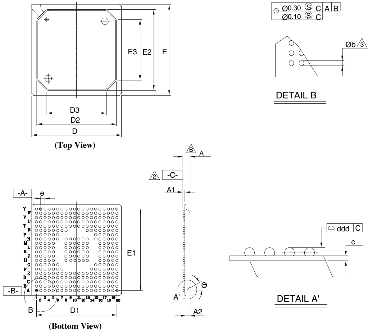
Figure 40. 352 Pin PBGA Pin Diagram
