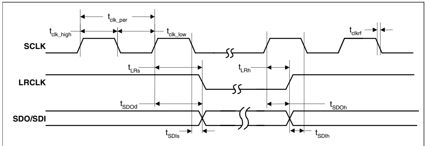
Figure 35. Inter-IC Sound (I 2 S) Timing Measurement
