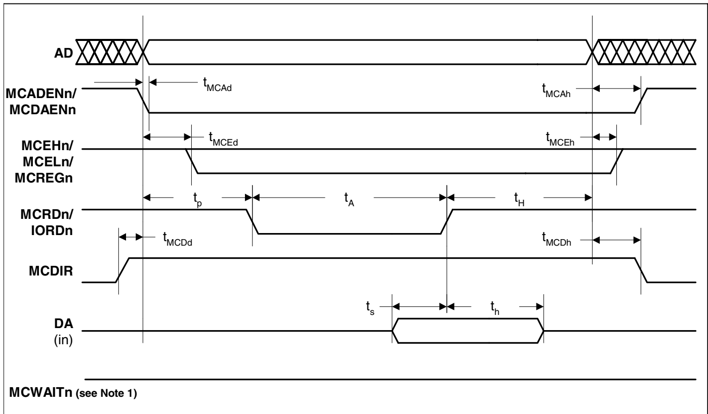
Figure 16. PCMCIA Read Cycle Timing Measurement
