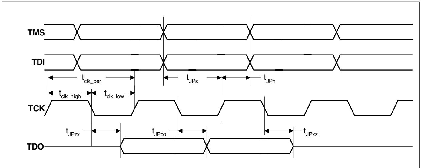
Figure 39. JTAG Timing Measurement
