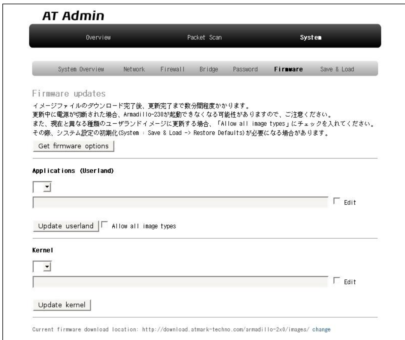
図 5-10 AT Admin: System – Firmware
