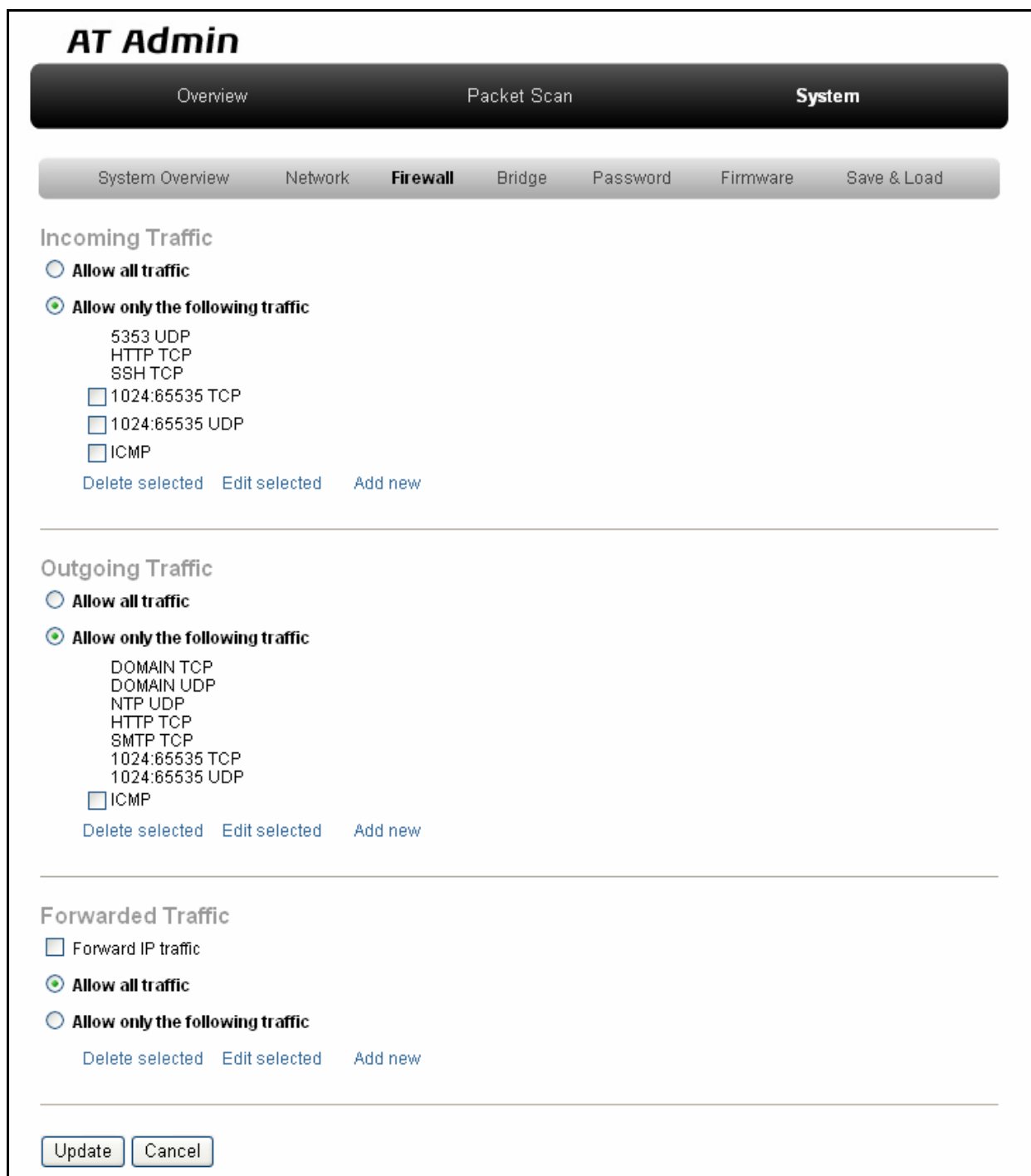
図 5-7 AT Admin: System – Firewall
