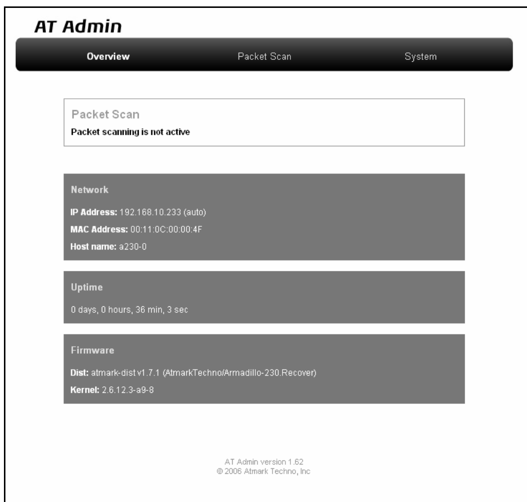
図 5-1 AT admin: Overview
