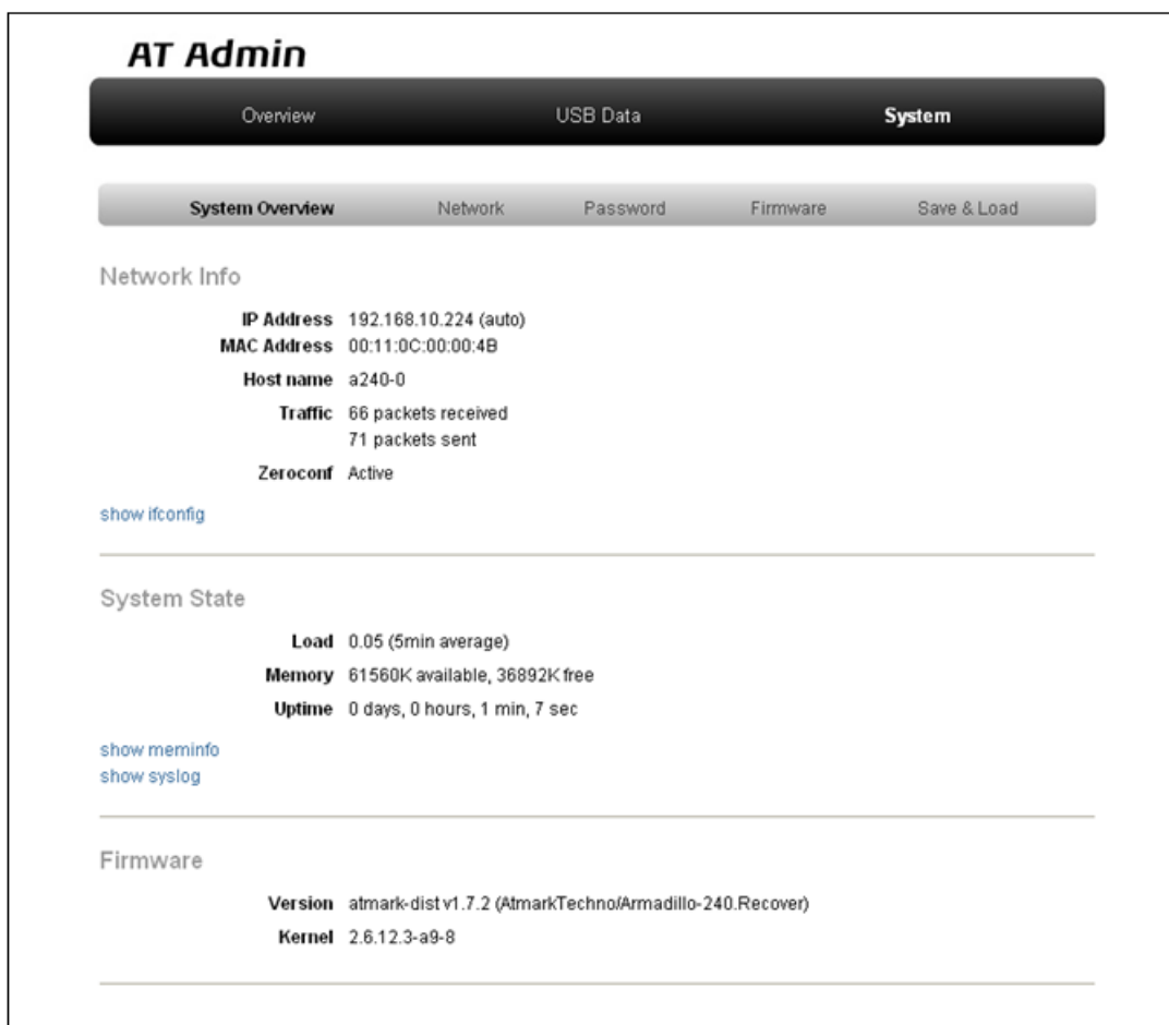
図 5.4. AT Admin: System - System Overview
