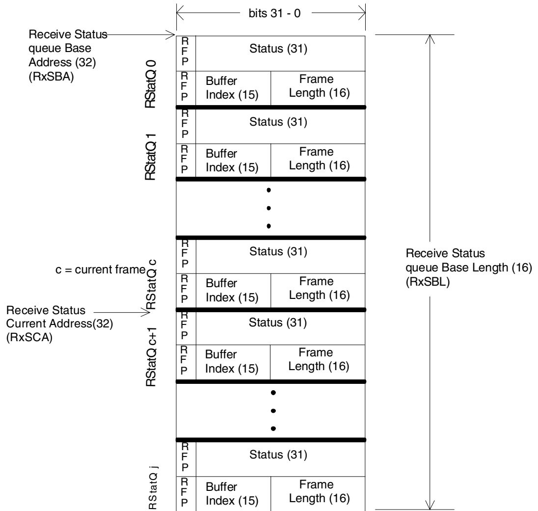
Figure 9-8. Receive Status Queue
