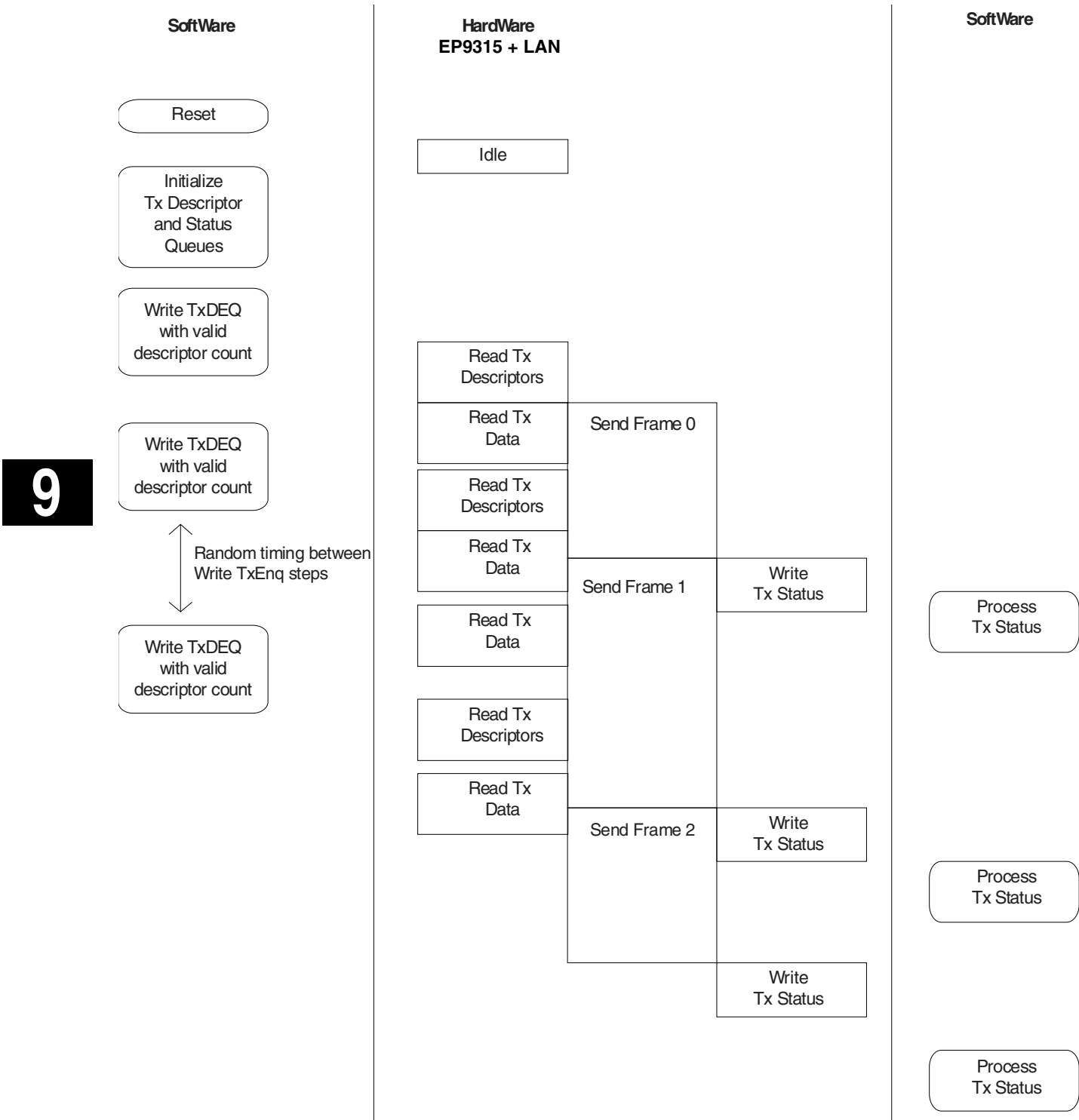
Figure 9-17. Transmit Descriptor Data/Status Flow
