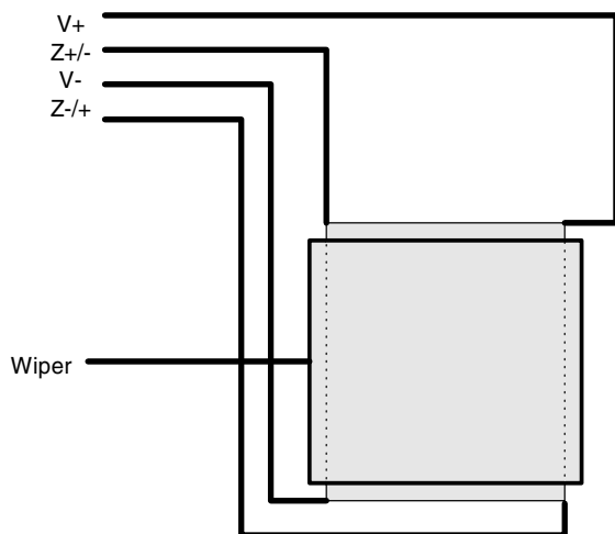
5 WIRE ANALOG RESISTIVE TOUCH SCREEN SCHEMATIC
