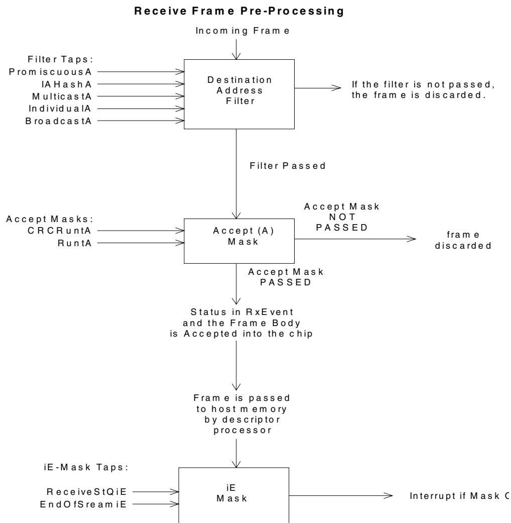
Figure 9-12. Receive Frame Pre-processing
