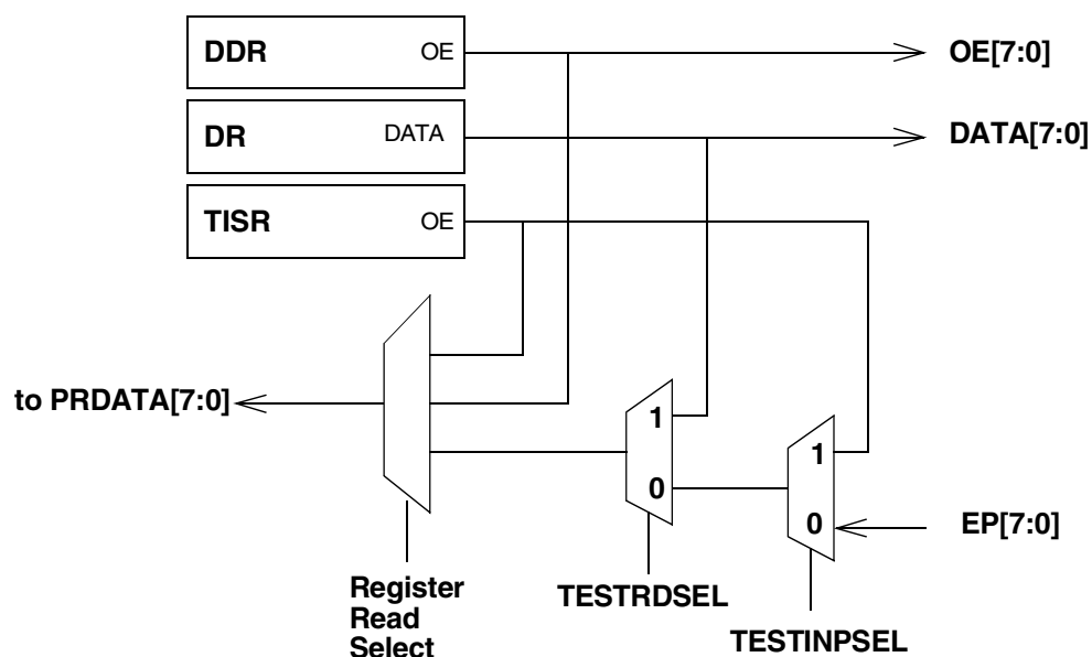
Figure 28-2. Signal Connections Within the Standard GPIO Port Control Logic (Ports C, D, E, G, H)
