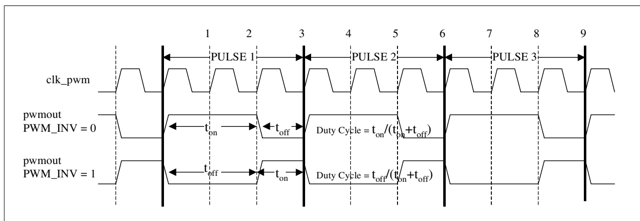
Figure 24-1. PWM_INV Example
