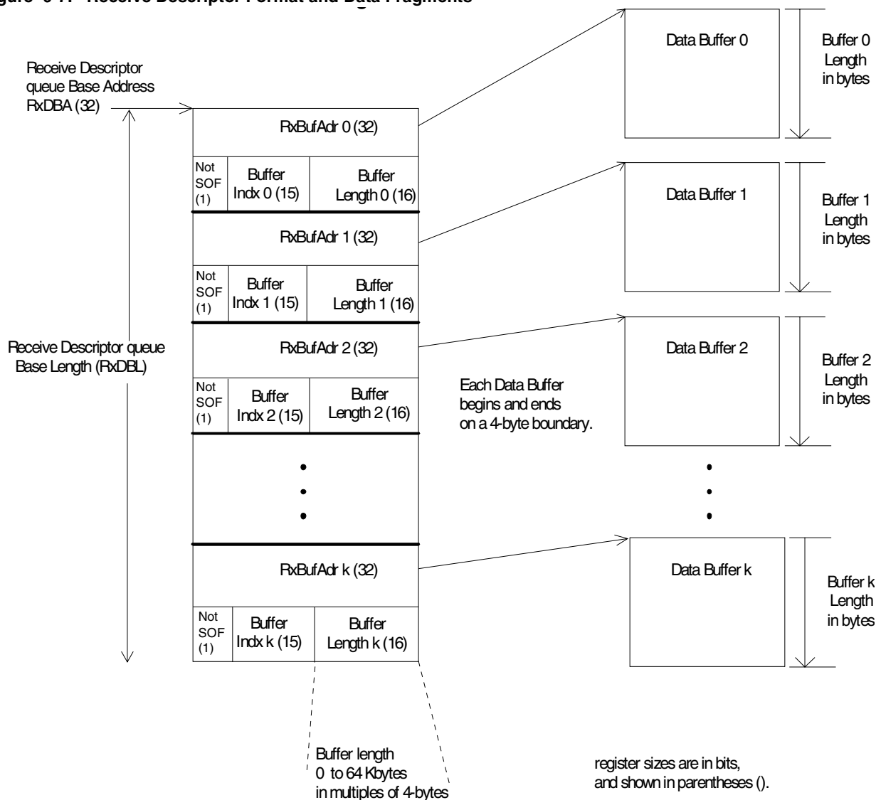
Figure 9-7. Receive Descriptor Format and Data Fragments
