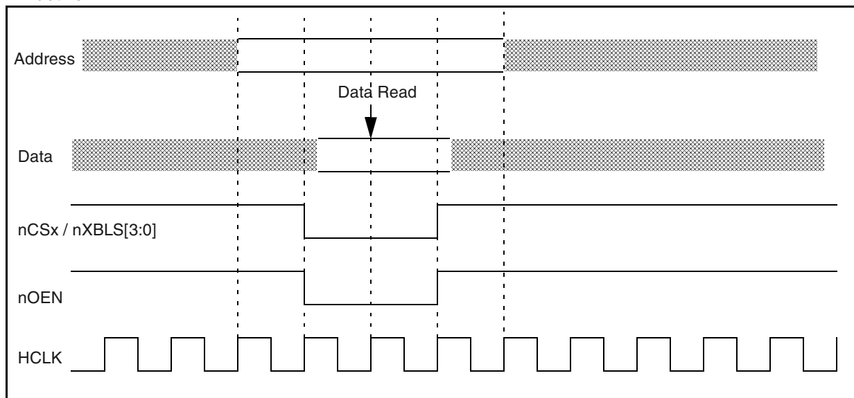
Figure 12-1. 32-bit read, 32-bit Memory, 0 wait cycles, RBLE = 1, WAITn Inactive
