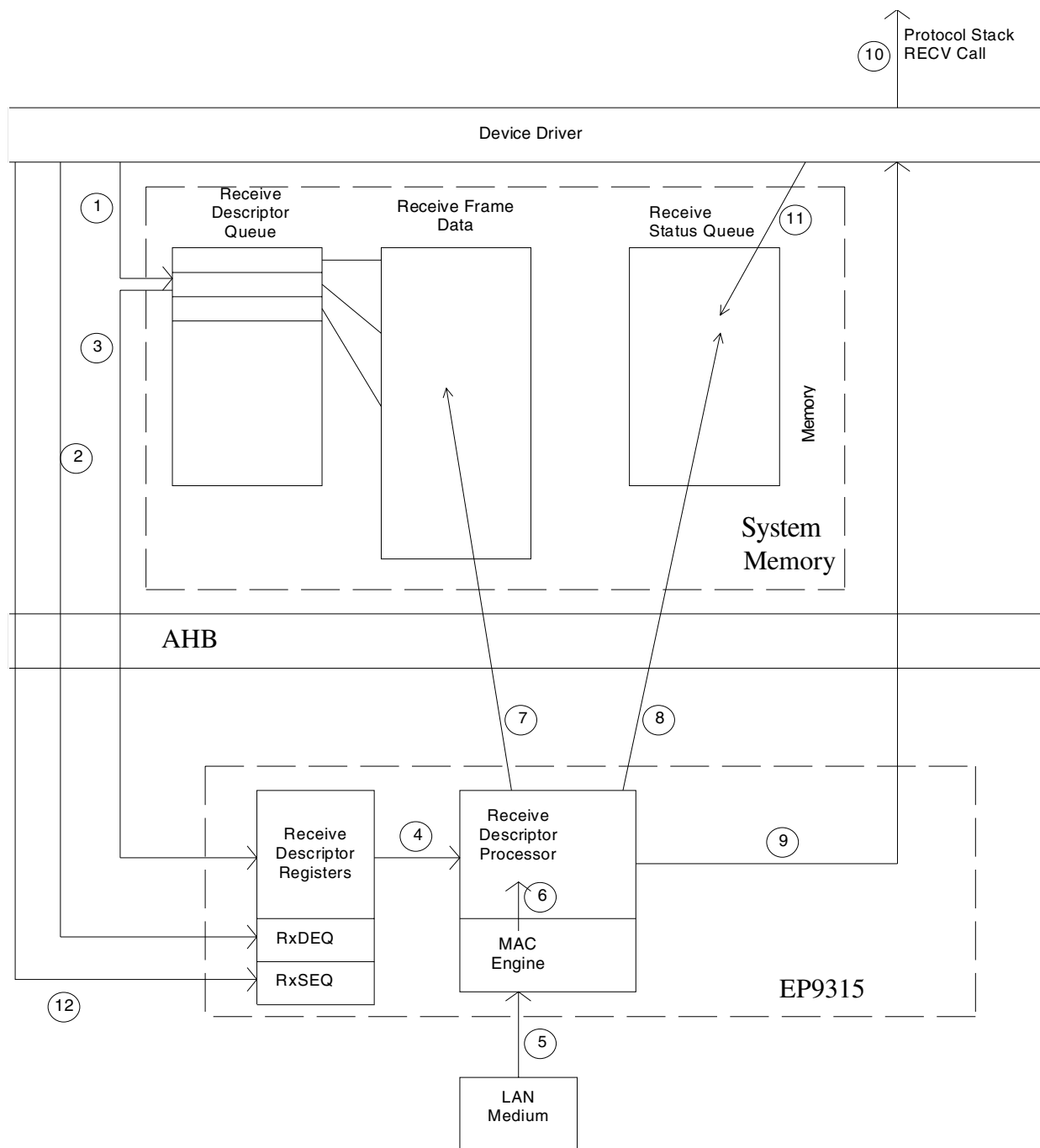
Figure 9-9. Receive Flow Diagram
