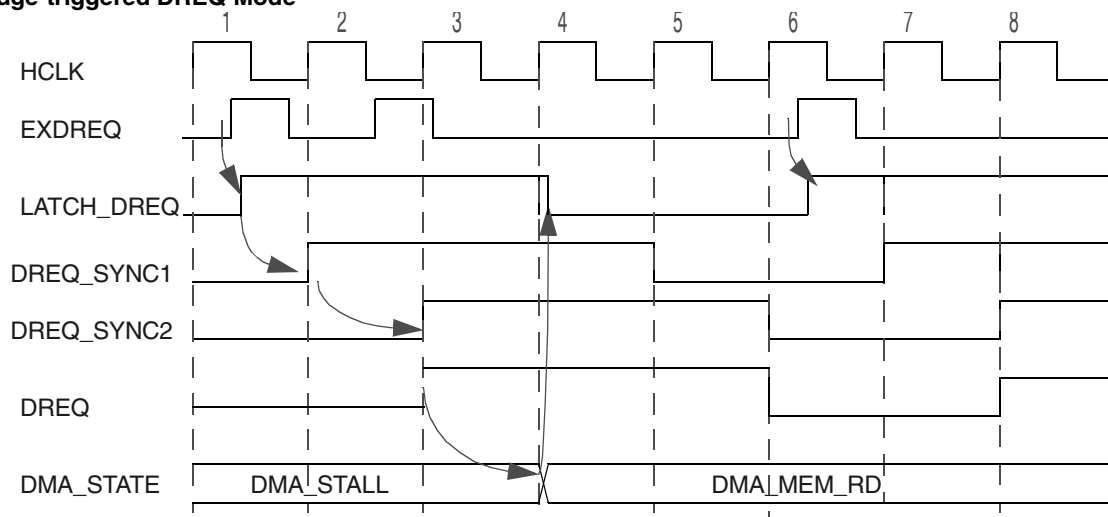
Figure 10-4. Edge-triggered DREQ Mode
