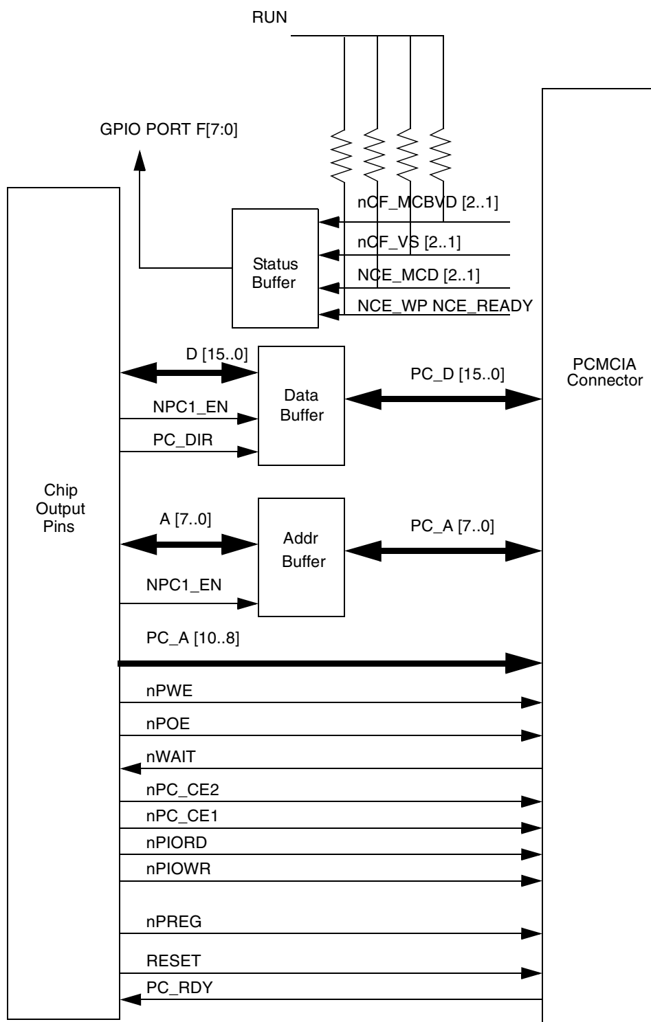
Figure 12-5. PCMCIA Single Card Interface
