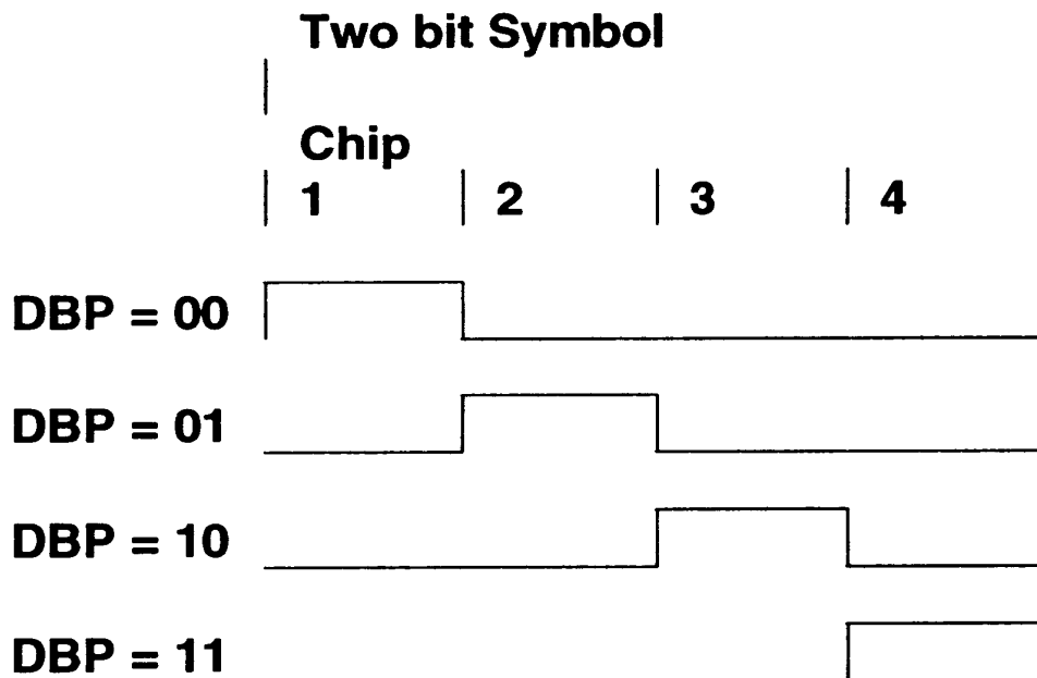
Figure 17-2. 4PPM Modulation Encoding
