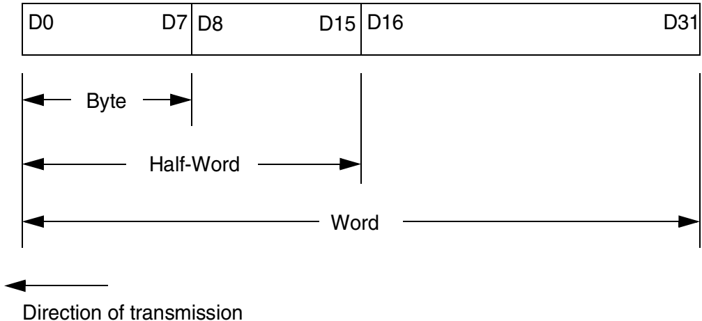
Figure 9-5. Data Bit Transmission Order
