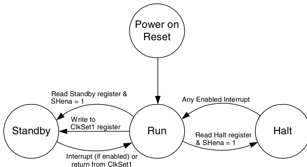
Figure 5-4. EP9315 Power States and Transitions
