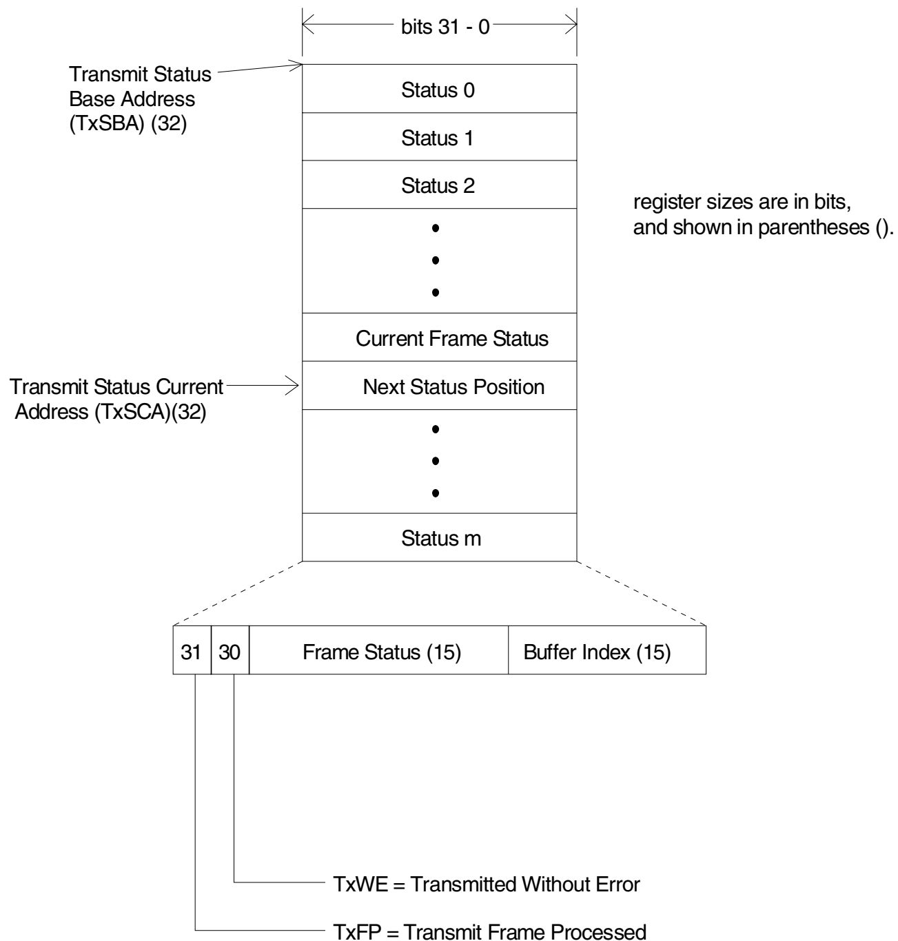
Figure 9-15. Transmit Status Queue
