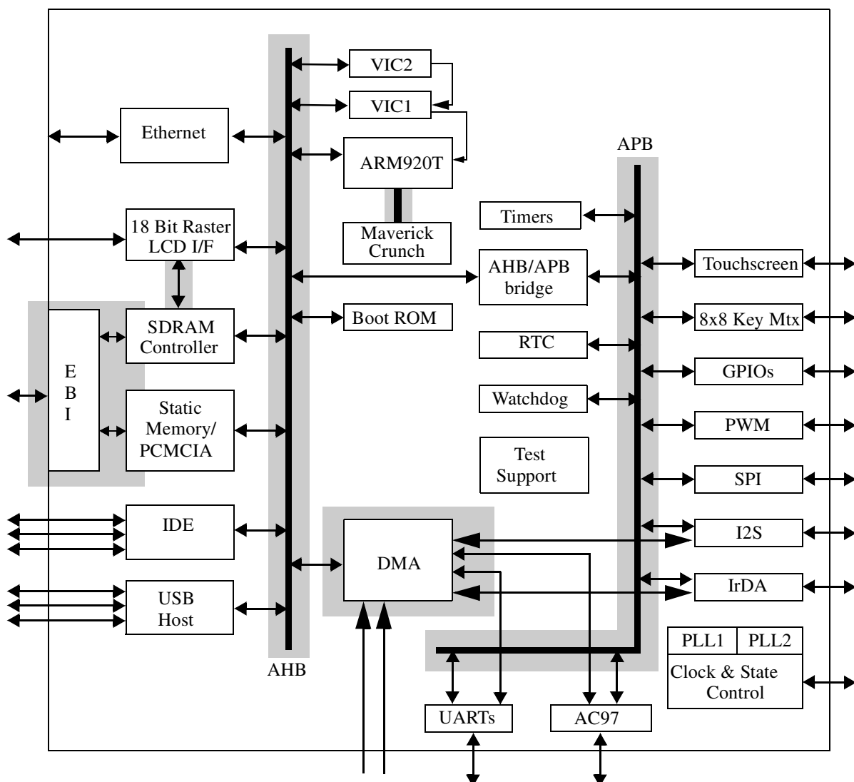
Figure 2-3. EP9315 Main Data Paths
