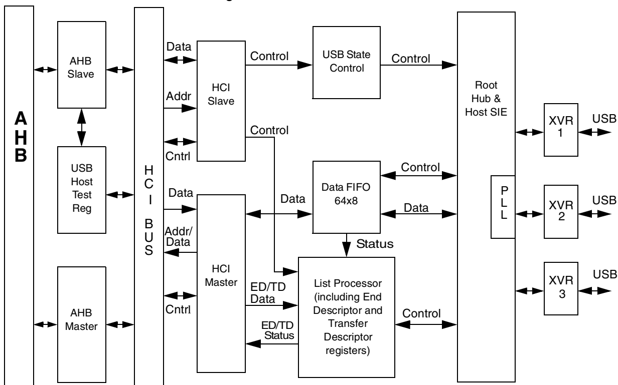
Figure 11-7. USB Host Controller Block Diagram
