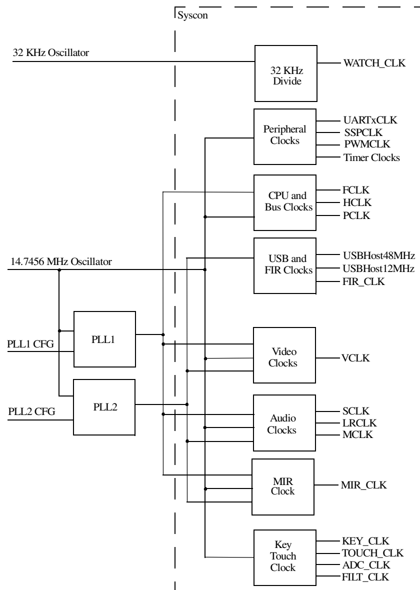
Figure 5-2. EP9315 Clock Generation System
