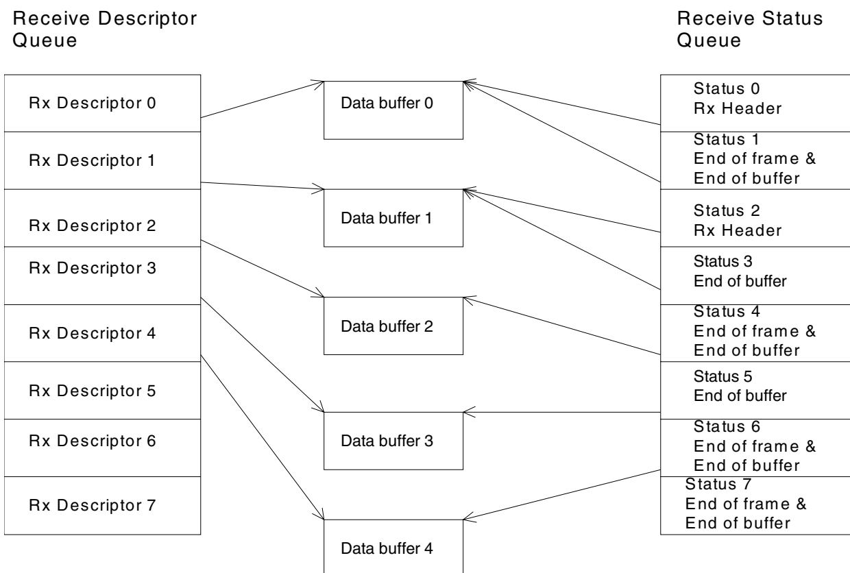
Figure 9-11. Receive Descriptor Example
