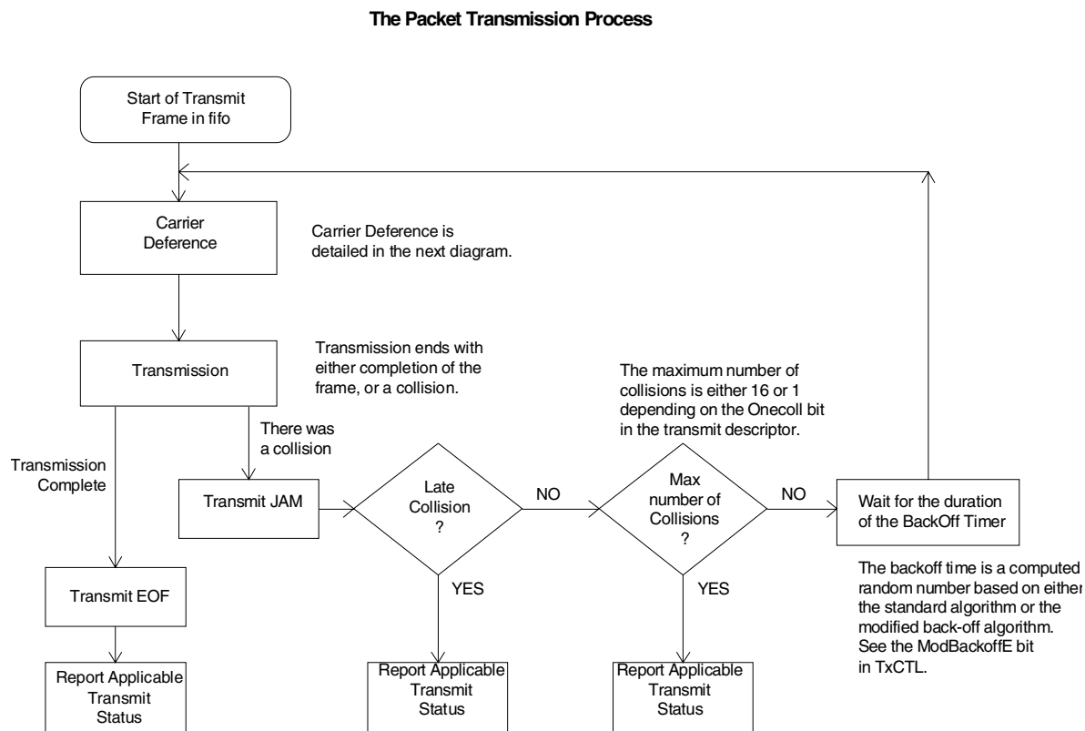
Figure 9-3. Packet Transmission Process
