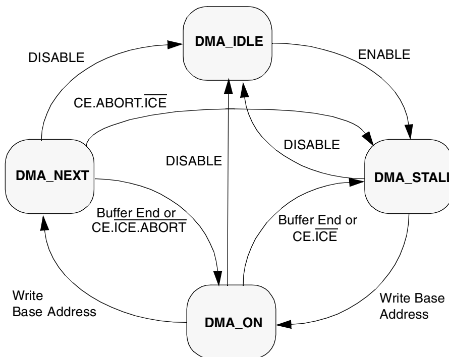
Figure 10-1. DMA M2P/P2M Finite State Machine
