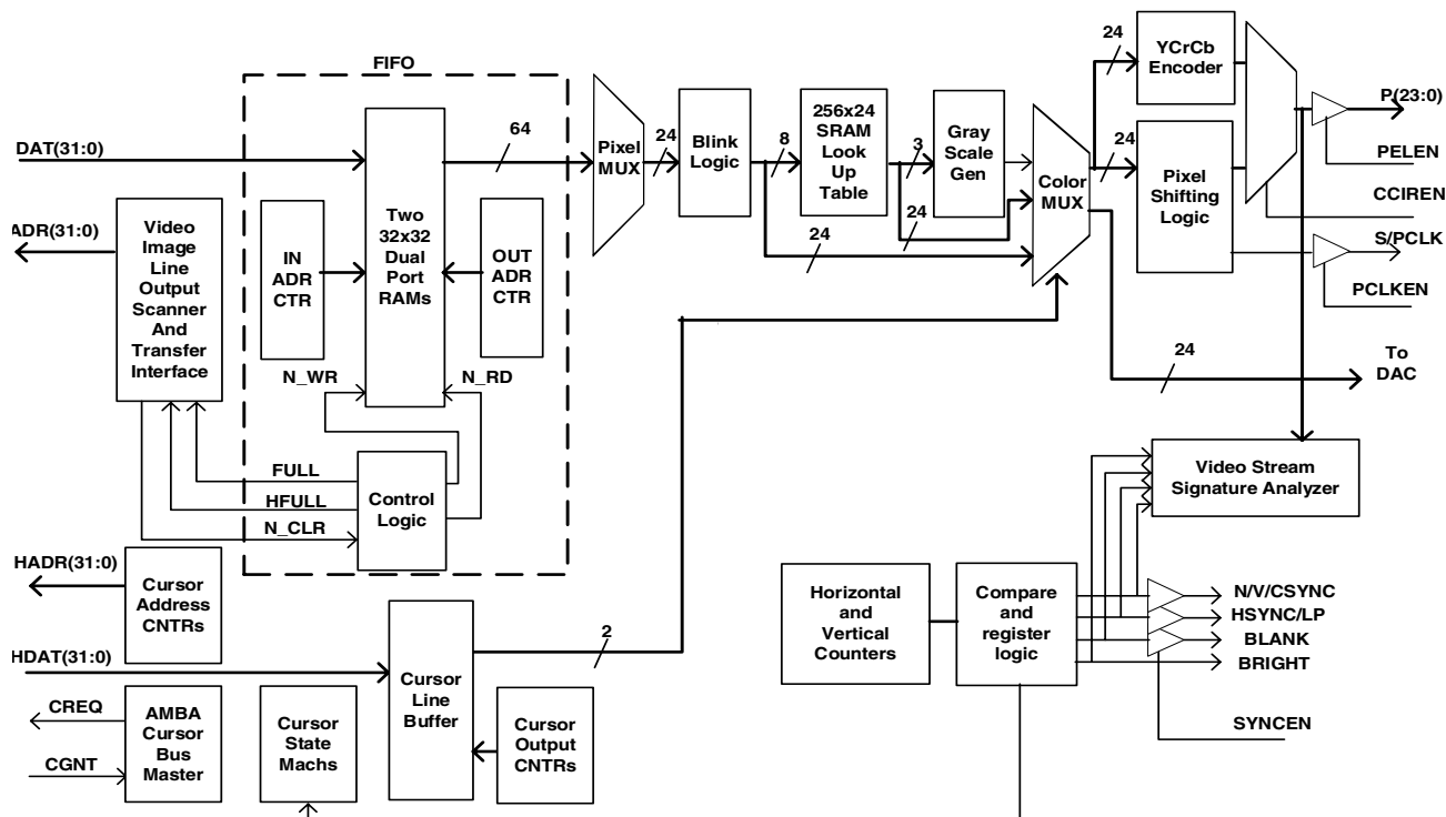
Figure 7-1. Raster Engine Block Diagram
