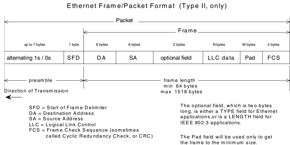
Figure 9-2. Ethernet Frame / Packet Format (Type II only)
